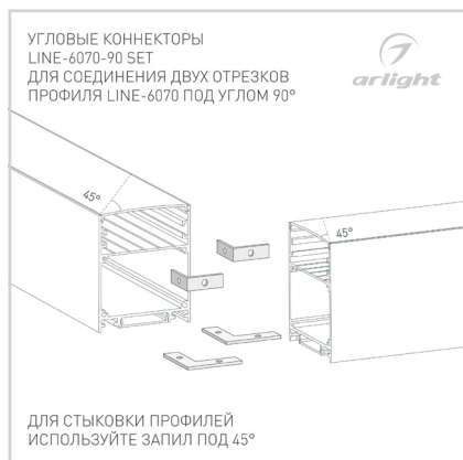
046862 LINE-6070-90 Set
